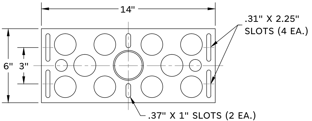
TOP VIEW
